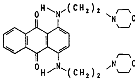
Compound 1d
